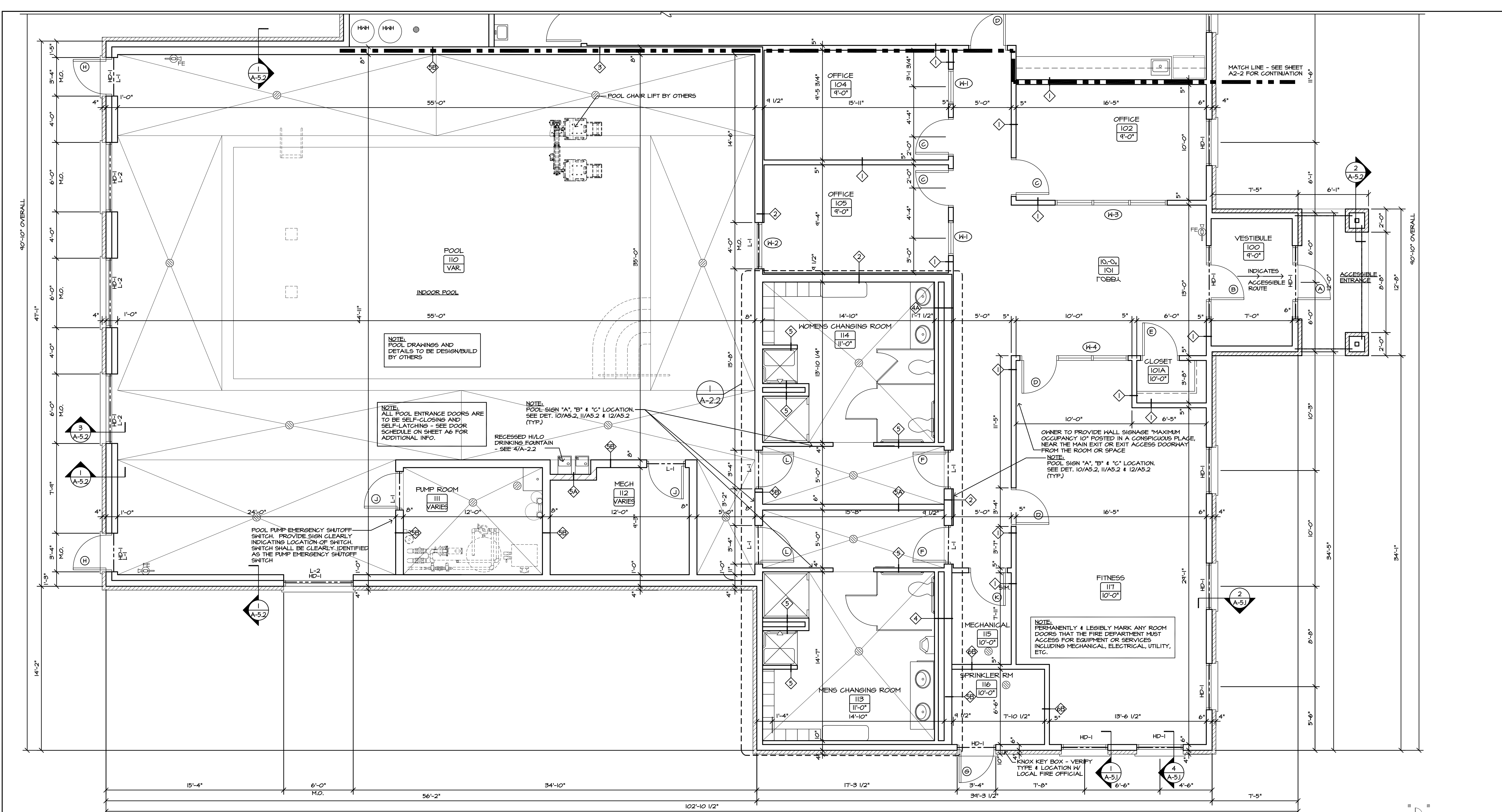
PARTIAL FLOOR PLAN SCALE: 1/4" = 1'-0" 7372 S.F.
